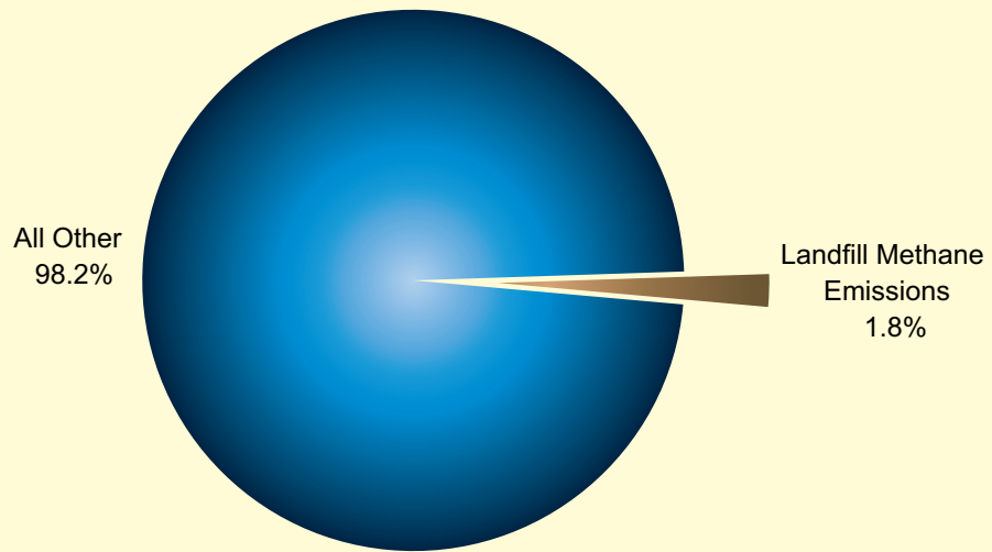
Figure 8: 100-Year Time Frame, Landfill Methane Emissions (% of total U.S. emissions in 2005, CO 2 eq.)
